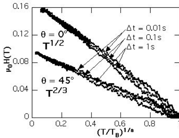
Fig. 3.5 Temperature dependence of the switching field of a 3 nm Co cluster as in Fig. 3.4 but plotted as a function of (T/T_B)^{1/a} with T_B = 14 K and a = 2 or 3/2 for \theta = 0^\circ and 45^\circ , respectively, and for three waiting times \Delta t .
