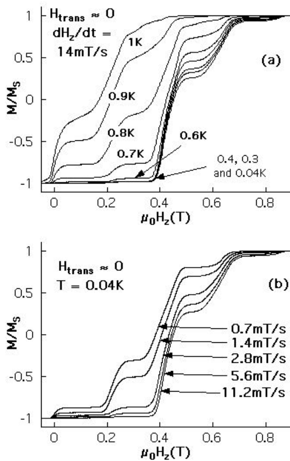
Fig. 4.4 Hysteresis loops of a single crystal of Fe 8 molecular clusters: (a) at different temperatures and a constant sweeping rate dH_z/dt = 0.014 \text{ T/s} , and (b) at 0.04 K and different field sweeping rates. The loops display a series of steps, separated by plateaus. As the temperature is lowered, there is a decrease in the transition rate due to reduced thermal assisted tunneling. The hysteresis loops become temperature independent below 0.35 K, demonstrating quantum tunneling at the lowest energy levels. The resonance widths at small fields H_z of about 0.05 T are mainly due to dipolar fields between the molecular clusters [118, 129].
