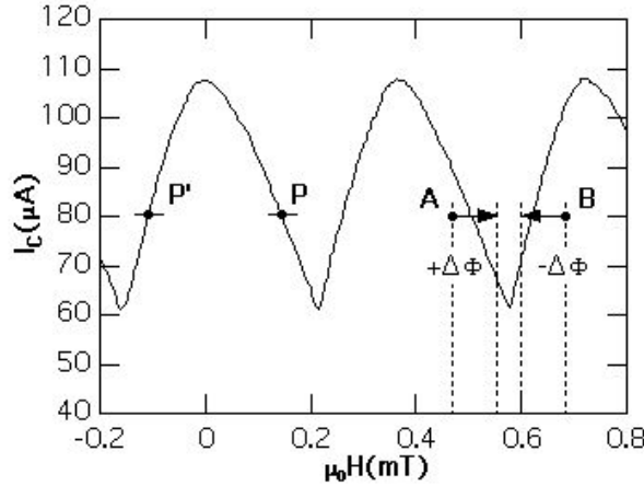
Fig. 1.4 Critical current I_c of a Al micro-SQUID as a function of a magnetic field applied perpendicular to the SQUID plane. For the feedback mode an external field perpendicular to the SQUID loop is applied which keeps the critical current constant at a working point, for example point P or P' . For the cold mode method the SQUID is biased close to the critical current so that it is in state A or B , respectively of positive or negative flux jumps induced by the magnetization reversal.
