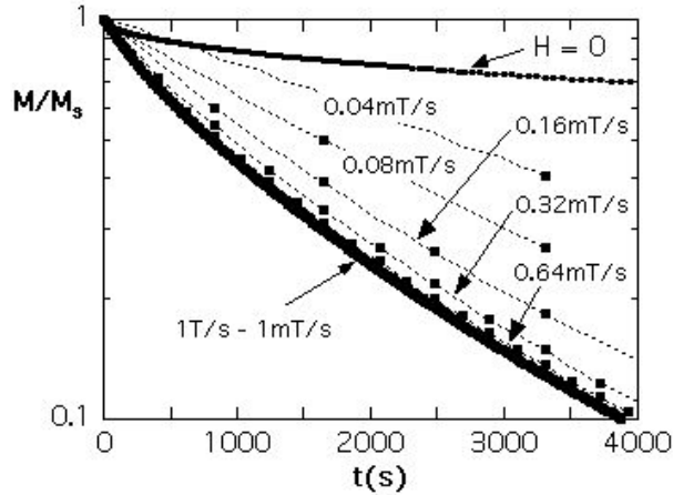
Fig. 4.7 Scaling plot for the Landau-Zener method showing the predicted field sweeping rate dependence for 1 T/s to 1 mT/s. Each point indicates the magnetization after a field sweep over the m = \pm 10 resonance. The dotted lines are guides for the eyes. For comparison, the figure displays also a relaxation curve at a constant field \vec{H} = 0 (Fig. 4.5) which shows much slower relaxation [129].
