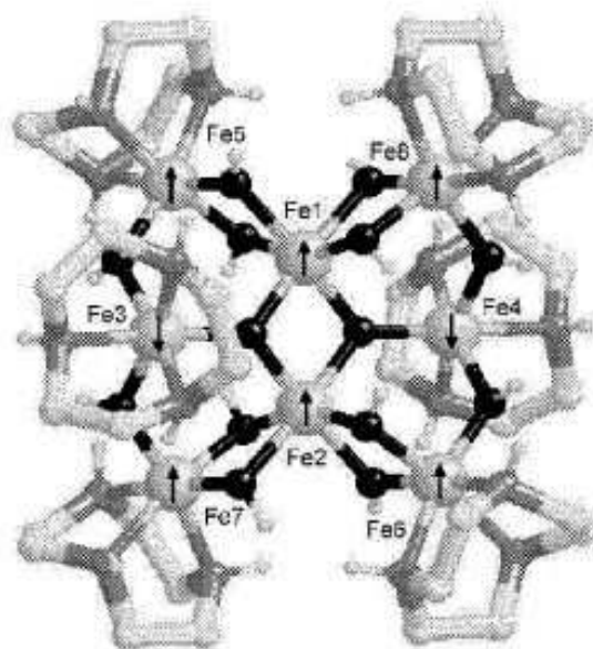
Fig. 4.1 Schematic view of the magnetic core of the Fe 8 cluster. The oxygen atoms are black, the nitrogen gray, and carbon atoms are white. For the sake of clarity only the hydrogen atoms that are exchanged with deuterium are shown as small spheres (Sect. 4.2.4). The arrows represent the spin structure of the ground state S = 10 as experimentally determined through polarized neutron diffraction experiments [109]. The exact orientation of easy, medium and hard axis of magnetization (Fig. 4.2) can be found in [110].
