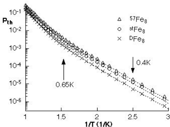
Fig. 4.19 Temperature dependencies of P_{th} for H_x = 0 for three \text{Fe}_8 samples. The field sweeping rate was 0.14 T/s. The dotted lines are fits of the data using Eq. 4.10.
