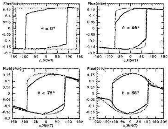
Fig. 2.3 Hysteresis loops of a nanocrystalline elliptic Co particle of 70 \times 50 \times 25 \text{ nm}^3 . The dashed line is the prediction of the Stoner–Wohlfarth model of uniform rotation of magnetization. The deviations are due to non uniform magnetization states.
