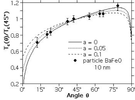
Fig. 4.21 Angular dependence of the crossover temperature T_c for a 10 nm \text{BaFe}_{10.4}\text{Co}_{0.8}\text{Ti}_{0.8}\text{O}_{19} particle with S \approx 10^5 . The lines are given by (4.11) for different values of the ratio a = H_\perp/H_\parallel . The experimental data are normalized by T_c(45^\circ) = 0.31 K
