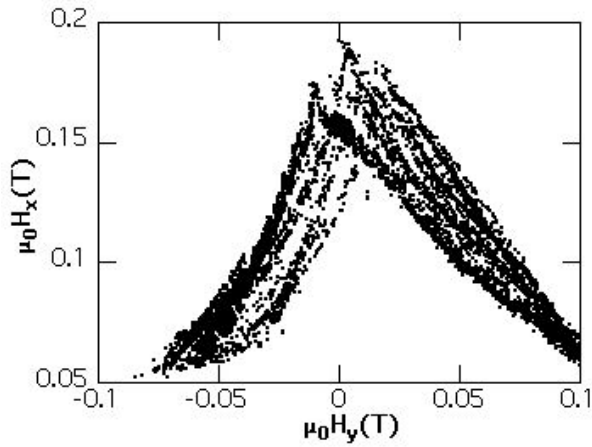
Fig. 3.6 Angular dependence of switching fields of a 3 nm Fe cluster having (probably) a slightly oxidized surface. Each point corresponds to one of the 10000 switching field measurement. The huge variations of the switching field might be due to exchange bias of frustrated spin configurations. However, quantum effects like those described in Sect. 4 are not completely excluded.
