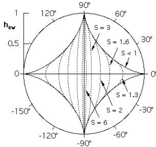
Fig. 2.12 Angular dependence of the switching field of an infinite cylinder for several reduced cylinder radii S . For S < 1 , the switching field is given by the uniform rotation mode (Sect. 2.1).
