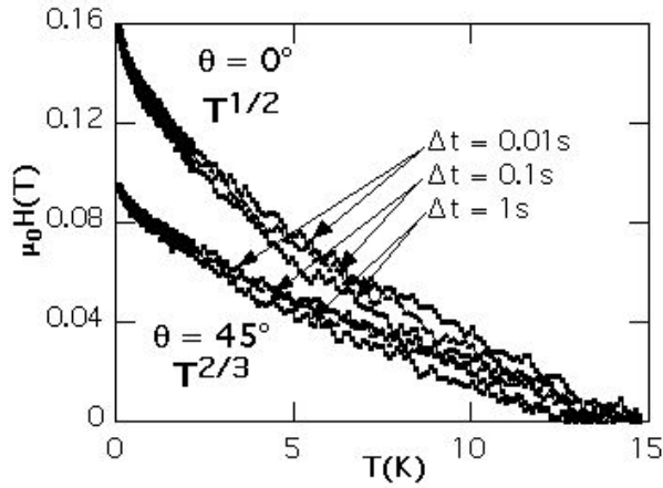
Fig. 3.4 Temperature dependence of the switching field of a 3 nm Co cluster, measured at 0^\circ and 45^\circ . The data were recorded using the blind mode method (Sect. 1.2.6) with different waiting time \Delta t of the applied field. The scattering of the data is due to stochastics and is in good agreement with Eq. 3.10.
