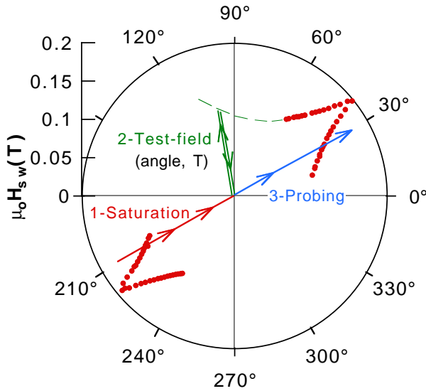
Fig. 1.7 Schematics for the blind mode method presenting the angular dependence of the switching field near the easy axis of a 3 nm Co cluster (full circles) (Sect. 2.1.2). First, the magnetization of the particle is saturated in a given direction (at T = 35 mK). Then, a test-field is applied, at a temperature between 35 mK and 30 K, which may or may not cause a magnetization switching. Finally, the SQUID is switched on (at T = 35 mK) and a field is applied in the plane of the SQUID to probe the resulting magnetization state.
