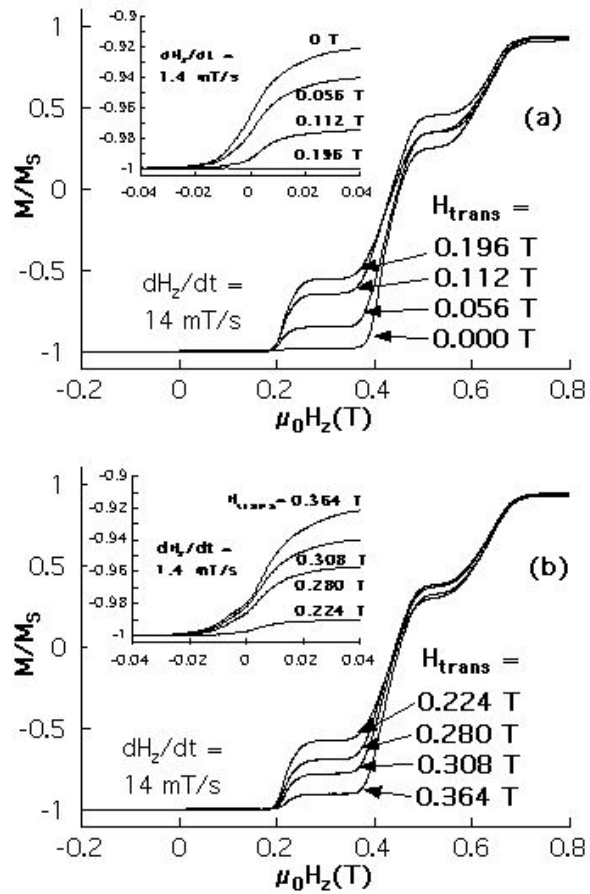
Fig. 4.5 Hysteresis loops measured along H_z in the presence of a constant transverse field at 0.04 K. Insets: enlargement around the field H_z = 0 . Notice that the sweeping rate is ten times slower for the measurements in the insets than that of the main figures.
