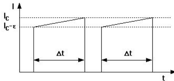
Fig. 1.3 Current injected into SQUID loop. First, the current is increased quickly up to a current I_c - \epsilon which is close to the critical current I_c . Then, the current is ramped up to I_c . As soon as a dV/dt pulse is detected at the SQUID due to the transition from the superconducting to the normal state the current is set to zero. I_c is proportional to the duration of the current ramp \Delta t . The repetition rate of the cycle is up to 10 kHz.
