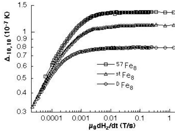
Fig. 4.8 Scaling plot for the Landau-Zener method showing the predicted field sweeping rate dependence for 1 T/s to 1 mT/s similar to Fig. 4.7 but for three isotopically substituted \text{Fe}_8 samples. Further details are presented in Sect. 4.2.4
