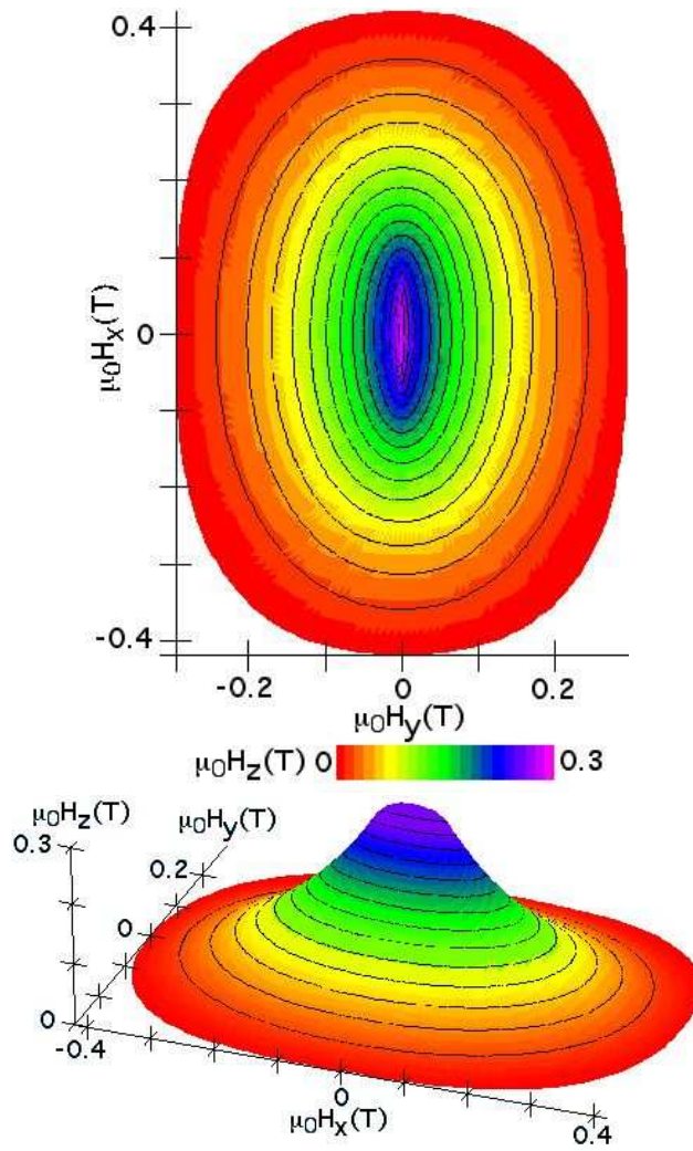
Fig. 2.7 Top view and side view of the theoretical switching field surface considering second and fourth order terms in the anisotropy energy.
