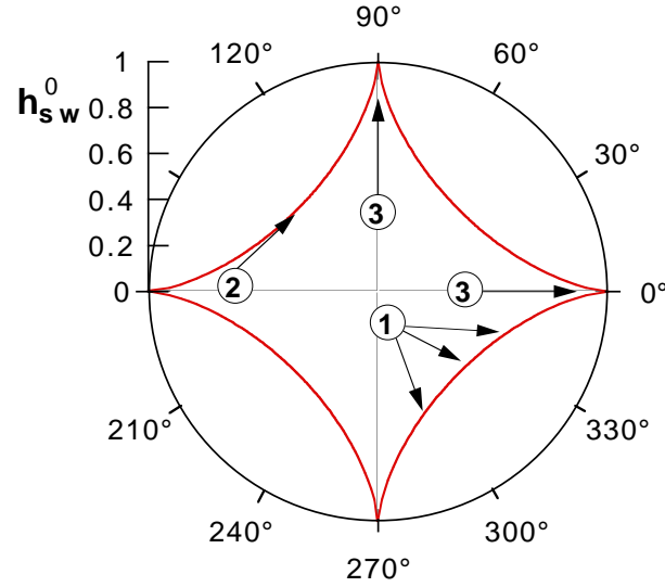
Fig. 2.1 Angular dependence of the Stoner-Wohlfarth switching field h_{sw}^0 = H_{sw}^0/H_a (Eq. 2.2). This curve is often called the ‘Stoner-Wohlfarth astroid’. The cases (1) to (3) correspond to Eqs. 2.5 to 2.9 concerning the field dependence of the anisotropy barrier height.
