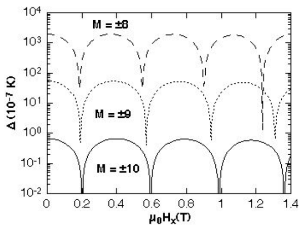
Fig. 4.16 Calculated tunnel splitting \Delta_{m,m'} as a function of the transverse field H_x for quantum transition between m = \pm 10, \pm 9 and \pm 8 (Sect. 4.1.3.2).
