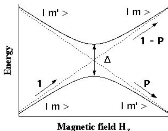
Fig. 4.6 Detail of the energy level diagram near an avoided level crossing. m and m' are the quantum numbers of the energy level. P_{m,m'} is the Landau-Zener tunnel probability when sweeping the applied field from the left to the right over the anti-crossing. The greater the gap \Delta and the slower the sweeping rate, the higher is the tunnel rate (Eq. 4.2).
