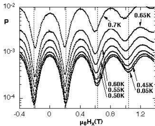
Fig. 4.15 Transverse field dependence of the tunneling probability P at several temperatures, and the ground state tunneling probability P_{-10,10} measured at T = 0.05 K and for {}^{st}\text{Fe}_8 . The field sweeping rate was 0.14 T/s. The dotted lines indicate the minima of P_{-10,10} .
