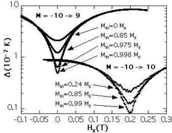
Fig. 4.14 Detailed measurement of the tunnel splitting \Delta around a topological quench for the quantum transition between m = -10 and (10 - n) at \varphi = 0^\circ . Note the strong dependence on the initial magnetization M_{in} which demonstrates the transverse dipolar interaction between \text{Fe}_8 molecular clusters [129].
