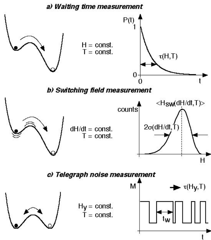
Fig. 3.1 Schema of three methods for studying the escape from a potential well: waiting time and telegraph noise measurements give direct access to the switching time probability P(t) , whereas switching field measurements yield histograms of switching fields
