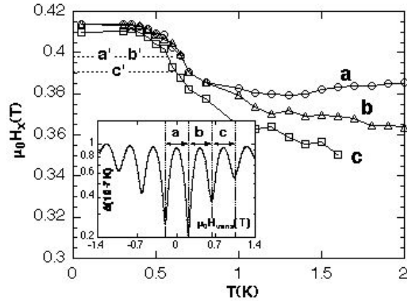
Fig. 4.17 Temperature dependence of the field between minima of the tunneling probability P in Fig. 4.15. a, b, and c are defined in the inset. The dotted line labeled with a', b', and c' where take from P_{th} of Fig. 4.18; see also [126].
