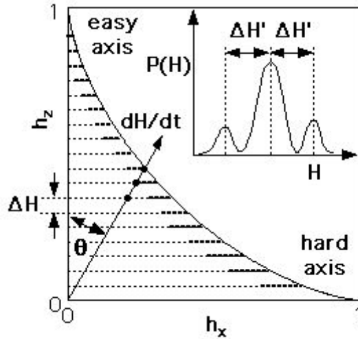
Fig. 4.22 Schematic view of the resonance fields of a giant spin S . The continuous line is the classical switching fields of Stoner–Wohlfarth (Sect. 2.1). The inset presents schematically a switching field histogram with \Delta H' \approx \frac{H_a}{2S} \frac{1}{\cos \theta}
