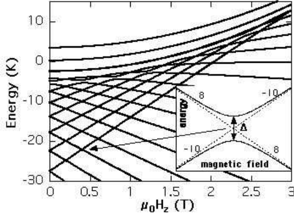
Fig. 4.3 Zeeman diagram of the 21 levels of the S = 10 manifold of \text{Fe}_8 as a function of the field applied along the easy axis (Eq. 4.1). From bottom to top, the levels are labeled with quantum numbers m = \pm 10, \pm 9, \dots, 0 . The levels cross at fields given by \mu_0 H_z \approx n \times 0.22 T, with n = 1, 2, 3, \dots . The inset displays the detail at a level crossing where the transverse terms (terms containing S_x or/and S_y spin operators) turn the crossing into an avoided level crossing. The greater the tunnel splitting \Delta , the higher the tunnel rate.
