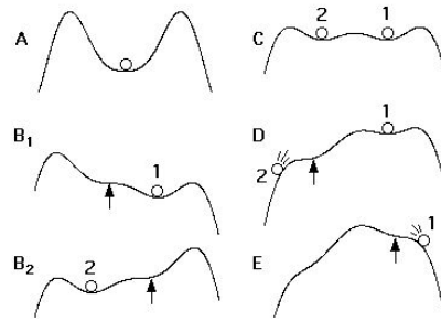
Fig. 2.10 Scheme of the potential energy near the metastable state for different applied fields as indicated in Fig. 2.9. The ball represent the state of the magnetization and the arrow locate the appearing or disappearing well.
