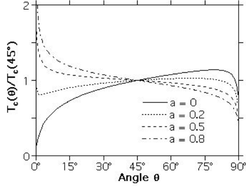
Fig. 4.20 Normalized crossover temperature T_c as given by (4.11), and for several values of the ratio a = H_{\perp}/H_{\parallel}
