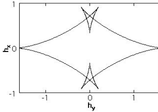
Fig. 2.8 Angular dependence of the switching field obtained from Eqs. 2.13 to 2.15 with K_1 > 0 and K_2 = -2/3K_1 . The field is normalized by the factor 2K_1/(\mu_0 M_s) .
