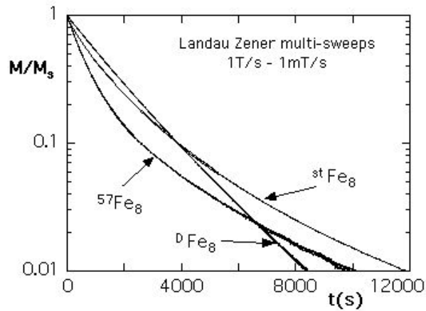
Fig. 4.9 Field sweeping rate dependence of the tunnel splitting \Delta_{-10,10} measured by a Landau-Zener method for three \text{Fe}_8 samples, for H_x = 0 . The Landau-Zener method works in the region of high sweeping rates where \Delta_{-10,10} is sweeping rate independent. Note that the differences of \Delta_{-10,10} between the three isotopically substituted samples are rather small in comparison to the oscillations in Fig. 4.10.
