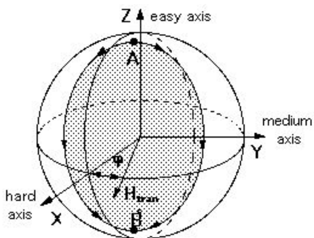
Fig. 4.2 Unit sphere showing degenerate minima A and B which are joined by two tunnel paths (heavy lines). The hard, medium, and easy axes are taken in x -, y - and z -direction, respectively. The constant transverse field H_{trans} for tunnel splitting measurements is applied in the xy -plane at an azimuth angle \varphi . At zero applied field \vec{H} = 0 , the giant spin reversal results from the interference of two quantum spin paths of opposite direction in the easy anisotropy yz -plane. For transverse fields in direction of the hard axis, the two quantum spin paths are in a plane which is parallel to the yz -plane, as indicated in the figure. By using Stokes theorem it has been shown [128] that the path integrals can be converted in an area integral, giving that destructive interference, that is a quench of the tunneling rate, occurs whenever the shaded area is k\pi/S , where k is an odd integer. The interference effects disappear quickly when the transverse field has a component in the y -direction because the tunneling is then dominated by only one quantum spin path.
