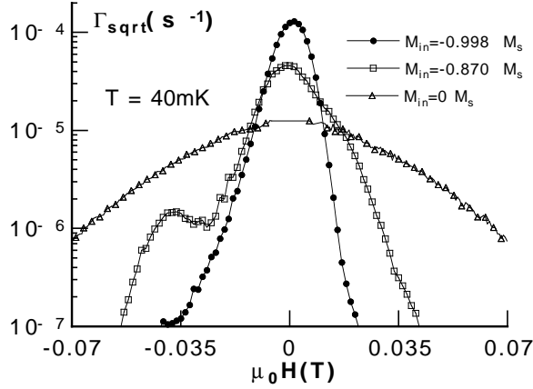
Fig. 4.13 Field dependence of the short time square-root relaxation rates \Gamma_{\text{sqrt}}(H_z) for three different values of the initial magnetization M_{\text{in}} . According to Eq. (4.6), the curves are proportional to the distribution P(H_z) of magnetic energy bias due to local dipole field distributions in the sample. Note the logarithmic scale for \Gamma_{\text{sqrt}} . The peaked distribution labeled M_{\text{in}} = -0.998M_s was obtained by saturating the sample, whereas the other distributions were obtained by thermal annealing. M_{\text{in}} = -0.870M_s is distorted by nearest neighbor lattice effects.
