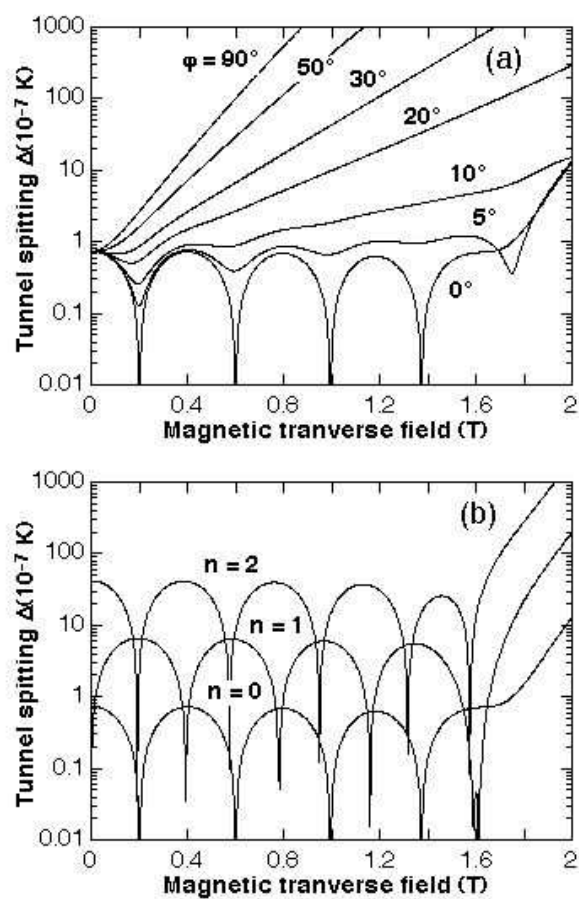
Fig. 4.11 Calculated tunnel splitting \Delta as a function of transverse field for (a) quantum transition between m = \pm 10 at several azimuth angles \varphi , and (b) quantum transition between m = -10 and (10 - n) at \varphi = 0^\circ (Sect. 4.1.3.2). The fourth order terms suppress the oscillations of \Delta for large transverse fields |H_x| .
