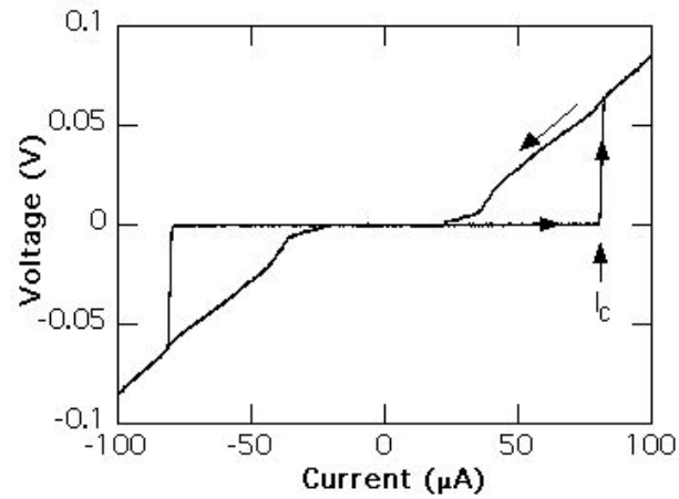
Fig. 1.2 Oscilloscope reading of a voltage versus current curve of a Nb micro-bridge-DC-SQUID. The SQUID transits from the superconducting to the normal state at the critical current I_c .
