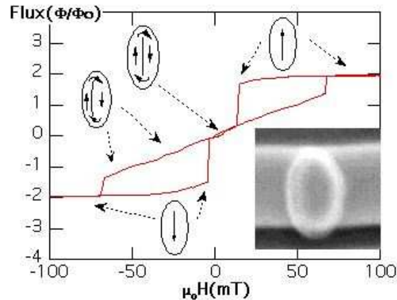
Fig. 2.14 Hysteresis loops at 0.1 K of the elliptic Co particle seen in the inset which shows the electron micrograph of the wire of a micro-bridge SQUID with the Co particle (300 nm \times 200 nm \times 30 nm). The in-plane field is applied along the long axis of the particles. The domain wall structure in an elliptical particle is also presented schematically as proposed by van den Berg. Arrows indicate the spin direction. The two small magnetization jumps near \approx \pm 5 mT might be due to the reversal of the center vortex of the domain structure.
