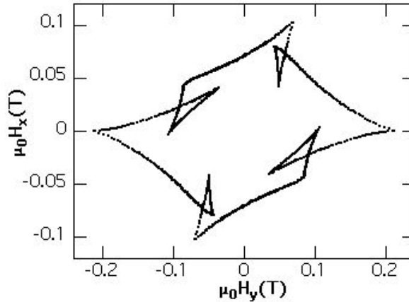
Fig. 2.11 Angular dependence of the switching field of a 3 nm Co cluster showing a strong influence of crystalline anisotropy.
