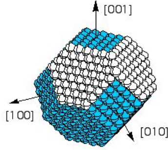
Fig. 2.5 Scheme of a typical cluster shape with light-gray atoms belonging to the 1289-atoms truncated octahedron basis and dark-gray atoms belonging to the (111) and (001) added facets.
