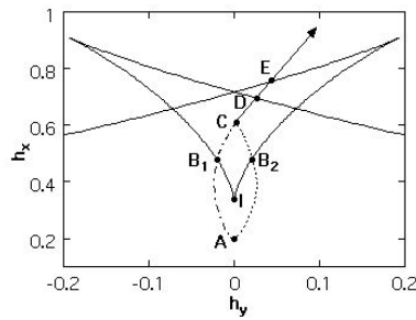
Fig. 2.9 Enlargement of angular dependence of the switching field of Fig. 2.8. Two possible paths of the applied field are indicated: starting from point A and going over the point B 1 leads to magnetization reversal in E whereas going over the point B 2 leads to reversal in D .
