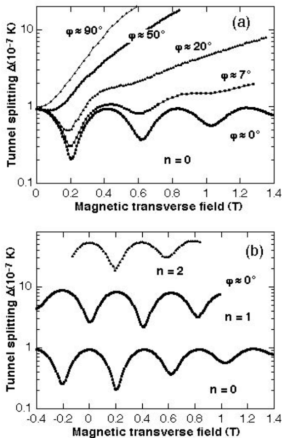
Fig. 4.10 Measured tunnel splitting \Delta as a function of transverse field for (a) several azimuth angles \varphi at m = \pm 10 , and (b) \varphi \approx 0^\circ , and for quantum transition between m = -10 and (10 - n) . Note the parity effect which is analogous to the suppression of tunneling predicted for half integer spins. It should also be mentioned that internal dipolar and hyperfine fields hinder a quench of \Delta which is predicted for an isolated spin (Figs. 4.11 and 4.14).
