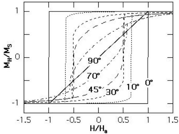
Fig. 2.2 Hysteresis loops of a Stoner-Wohlfarth particle for different field angles \theta . The component of magnetization along the direction of the applied field is plotted, i.e. , M_H = M_S \cos(\phi - \theta) .
