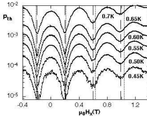
Fig. 4.18 Transverse field dependence of P_{th} which is the difference between the measured tunnel probability P and the ground state tunnel probability n_{-10}P_{-10,10} measured at T = 0.05K (see Fig. 4.15. The field sweeping rate was 0.14 T/s. The long dotted lines indicate the minima of P_{th} whereas the short dotted lines indicate the minima of P_{-10,10} .
