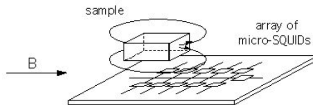
Fig. 1.8 Schematic representation of our magnetometer which is an array of micro-SQUIDs. Its high sensitivity allows us to study single crystals of the order of 10 to 500 \mu\text{m} which are placed directly on the array.
