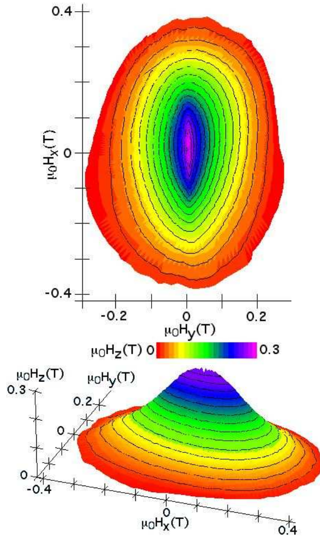
Fig. 2.6 Top view and side view of the experimental three dimensional angular dependence of the switching field of a 3 nm Co cluster at 35 mK. This surface is symmetrical with respect to the H_x - H_y -plane and only the upper part ( \mu_0 H_z > 0 T) is shown. Continuous lines on the surface are contour lines on which \mu_0 H_z is constant.
