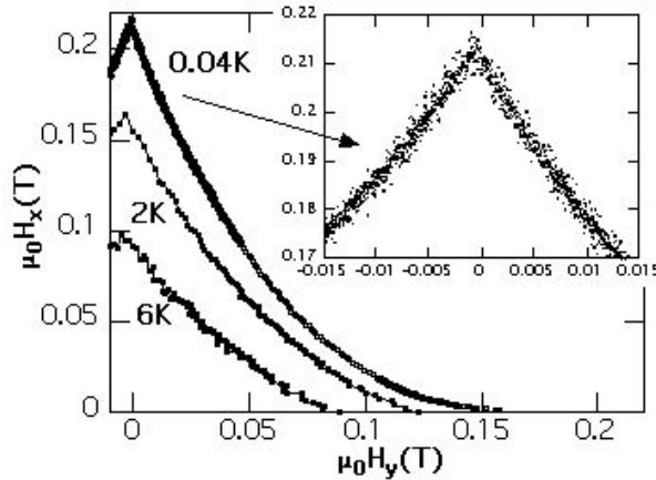
Fig. 4.23 Angular dependence of the switching field of a 3 nm Fe cluster with S \approx 800 . The inset presents detailed measurements near the easy axis of magnetization.
