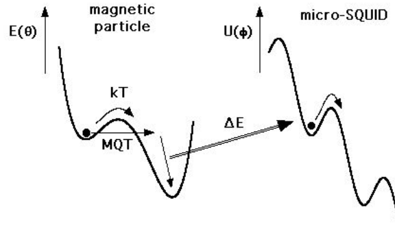
Fig. 1.6 Energy scheme of the cold mode method. After the particle overcomes the saddle point or tunnels through the energy barrier, it falls into the lower potential well releasing energy. A very small fraction \Delta E of this energy is transferred to the SQUID and drives the SQUID out of its metastable superconducting state.
