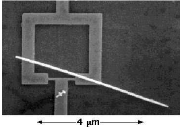
Fig. 1.1 Scanning electron micrograph of a Nb micro-bridge-DC-SQUID fabricated by electron beam lithography. A Ni wire of diameter of about 90 nm was deposit on the SQUID (Sect. 2.2.2).
