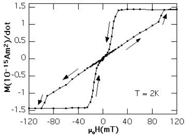
Fig. 2.15 Hysteresis loops of the magnetic moment of the array of 1.8 \times 10^7 Co particles ( 300 \text{ nm} \times 200 \text{ nm} \times 30 \text{ nm} ). The in-plane field is applied along the long axis of the particles.
