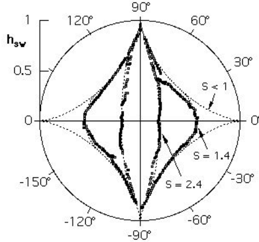
Fig. 2.13 Angular dependence of the switching field of two Ni wires with a diameter of 45 nm and 92 nm, i.e. S = 1.4 and 2.4 . The switching fields are normalized by 125 mT and 280 mT respectively.
