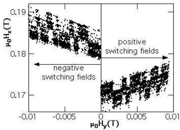
Fig. 3.7 Detail of the angular dependence of switching fields of a 3 nm Fe cluster having (probably) a slightly oxidized surface. Each point corresponds to one of the 3000 switching field measurement. Stochastic fluctuation between different switching field distributions are observed. The 'mean' hysteresis loop is shifted to negative fields.
