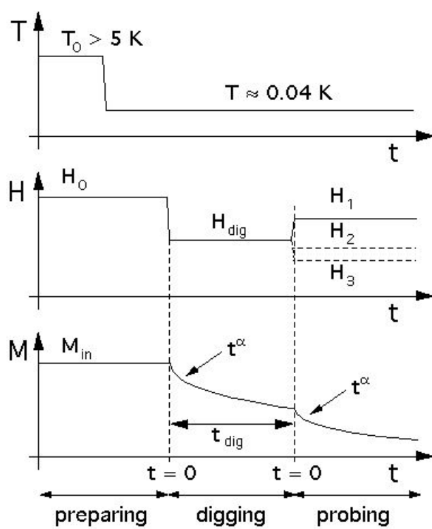
Fig. 4.12 Schema of the hole digging method presenting the time dependence of temperature, applied field and magnetization of the sample.
