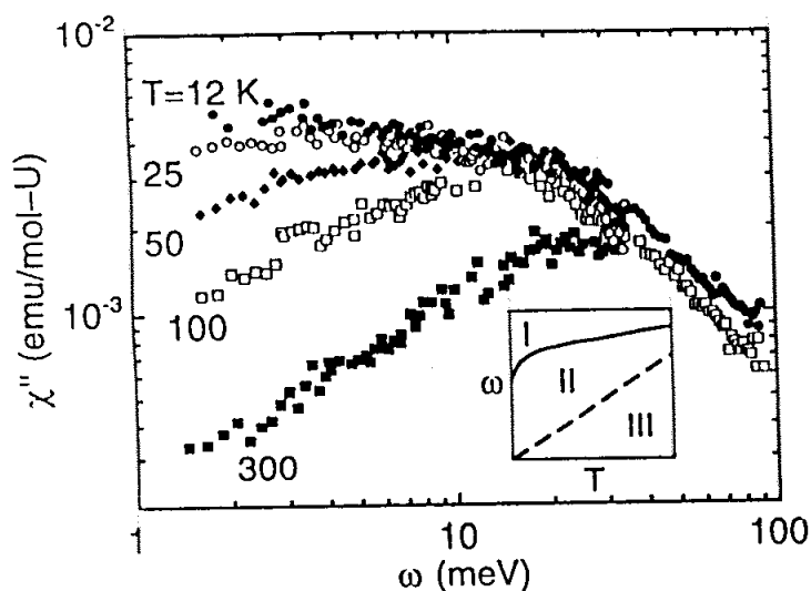
Fig. 15. \chi''(\omega) for \text{UCu}_4\text{Pd} at constant temperatures ranging from 12 K to 300 K. Inset: three qualitatively different regimes are observed in the response: I. \omega \geq \omega^* : \chi''(\omega, T) \sim (\omega/T_0) / [1 + (\omega/T_0)^2] . II. \omega \ll T : \chi''(\omega, T) \sim \omega/T^\eta , \eta = 1 \pm 1/3 . III. \omega \gg T : \chi''(\omega, T) \sim \omega^{-1/3} . Solid line: \omega^*(T) , dashed line: \omega = T . From Ref. 33
