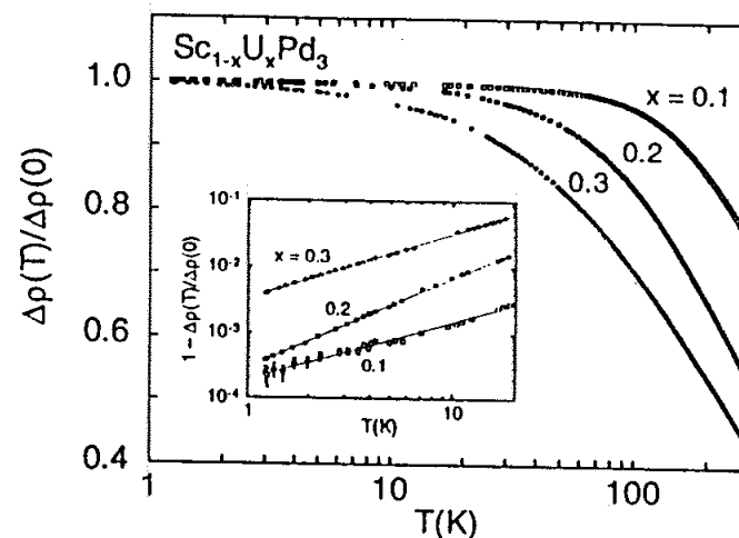
Fig. 3. Uranium contribution to the electrical resistivity \Delta\rho(T) of Sc_{1-x}U_xPd_3 ( x = 0.1, 0.2, 0.3 ), normalized to the extrapolated zero temperature value \Delta\rho(0) , versus \log T . Inset: Log-log plot of 1 - \Delta\rho(T)/\Delta\rho(0) = a(T/T_K)^n with n = 0.9 \pm 0.2, 1.4 \pm 0.2, \text{ and } 1.0 \pm 0.2 for x = 0.1, 0.2, \text{ and } 0.3 , respectively. From Ref. 10.
