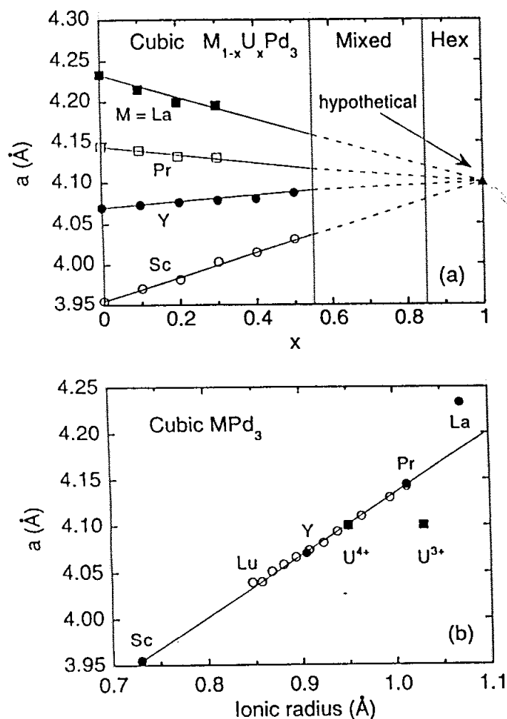
Fig. 2. (a) Cubic lattice parameters of M_{1-x}U_xPd_3 compounds as a function of x . Solid lines represent linear fits to the data, which extrapolate (dashed lines) to a common value of 4.100 \pm 0.005 \text{ \AA} for hypothetical cubic UPd_3 . (b) Lattice parameters of cubic MPd_3 compounds versus ionic radius of the trivalent ion. With the exception of LaPd_3 , the data fall on a straight line. The hypothetical value for cubic UPd_3 obtained from (a) (filled triangle) is consistent with U being tetravalent in the M_{1-x}U_xPd_3 compounds. From Ref. 8.
