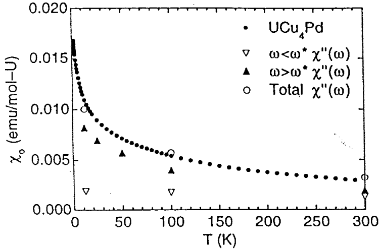
Fig. 17. A Comparison of the measured static susceptibility \chi(T) to that calculated from the measured dynamical susceptibility (see text) for energy transfers larger (filled triangles) and smaller (open triangles) than \omega^* = 25 meV. Integrating over the total response for 1 \text{ meV} \leq \omega \leq 200 \text{ meV} (open circles) accounts for virtually the entire measured \chi(T) .
