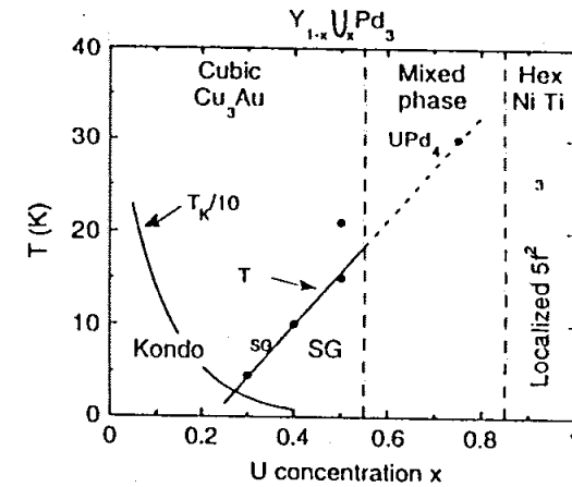
Fig. 1. Low temperature - U concentration phase diagram of Y_{1-x}U_xPd_3 . From Ref. 2.
