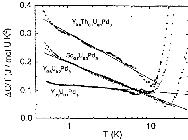
Fig. 5. Low temperature specific heat \Delta C/T versus \log T for various Kondo alloys which exhibit a T = 0 logarithmic divergence, a non Fermi liquid behavior. Solid lines are fits of the data to the two channel, S = 1/2 Kondo model plus a constant B' : \Delta C/T = -(0.251/T_K)R \ln(T/0.41T_K) + B' . The associated entropy suggests a finite zero temperature entropy of S(0) \approx (R/2) \ln(2) . From Ref. 8.
