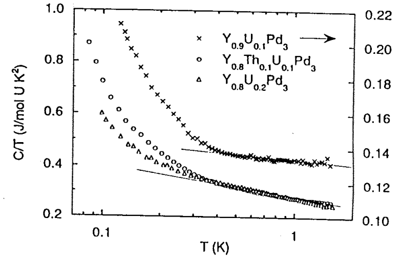
Fig. 6. Specific heat C/T versus \log T to temperatures as low as 80 mK for three of the Kondo alloys from Fig. 5, measured in a ^3\text{He}-^4\text{He} dilution refrigerator. Solid lines are fits of the data to the two channel, S = 1/2 Kondo model plus a constant B' .
