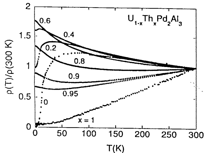
Fig. 10. Electrical resistivity \rho(T) , normalized to its room temperature value \rho(300 \text{ K}) , versus temperature T for the U_{1-x}Th_xPd_2Al_3 system for various values of x between 0 and 1.
