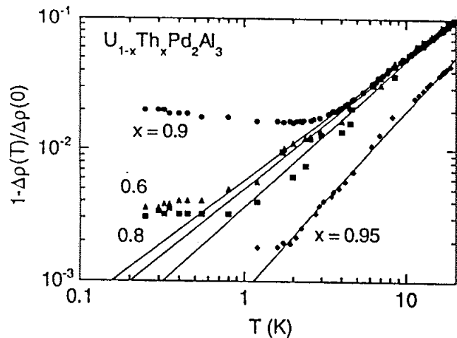
Fig. 11. Low temperature electrical resistivity data ( T \leq 20 \text{ K} ) plotted as \log(1 - \Delta\rho(T)/\Delta\rho(0)) versus \log T . Solid lines represent fits to a power law \Delta\rho(T)/\Delta\rho(0) = 1 - a(T/T_K)^n , with n \approx 1 , indicative of NFL behavior.
