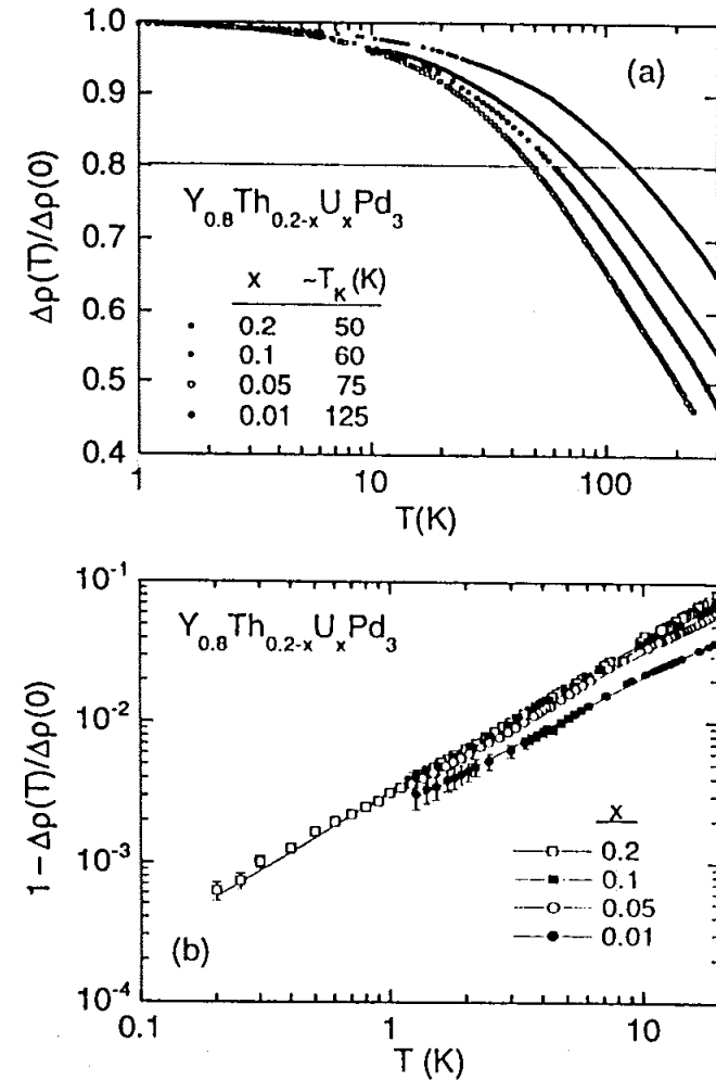
Fig. 4. (a) Normalized electrical resistivity \Delta\rho(T)/\Delta\rho(0) versus \log T for the Y_{0.8}Th_{0.2-x}U_xPd_3 ( 0 \leq x \leq 0.2 ) system revealing Kondo behavior with a Kondo temperature T_K which increases only slightly with decreasing x . (b) Low temperature resistivity data ( T \leq 20 K) plotted as \log(1 - \Delta\rho(T)/\Delta\rho(0)) versus \log T . Solid lines represent fits to a power law \Delta\rho(T)/\Delta\rho(0) = 1 - a(T/T_K)^n , with n = 1.0 \pm 0.1 for all samples, exhibiting NFL behavior. This value is in between that expected for single channel ( n = 2 ) and two channel ( n = 1/2 ) S = 1/2 Kondo models. From Ref. 8.
