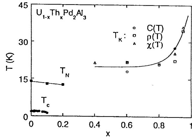
Fig. 9. Low temperature phase diagram of the U_{1-x}Th_xPd_2Al_3 system. As the Th concentration x is increased, the Neel temperature T_N and the superconducting critical temperature T_c decrease slightly, but the features associated with AFM and superconductivity are rapidly suppressed and eventually become undetectable. The line in the right hand side of the figure represents the estimated value of the Kondo temperature T_K .
