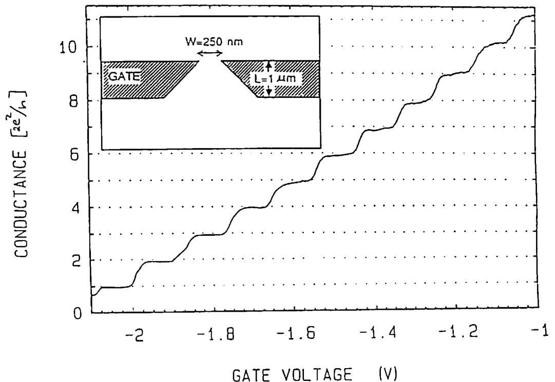
Fig. 5. Conductance of a semiconductor point contact as a function of gate voltage which controls the size of the constriction; inset shows schematic of the structure. Adapted from [31].
